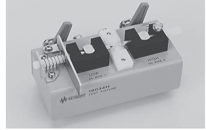
16034H SMD/chip test fixture
