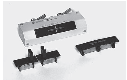
16047A axial & radial test fixture
